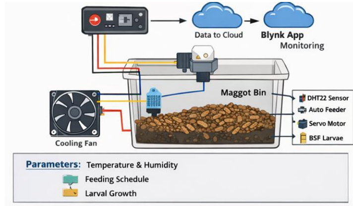
Figure 3. Experimental Setup
