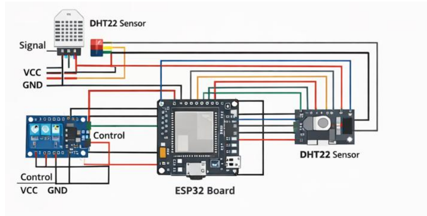
Figure 2. Hardware Wiring
