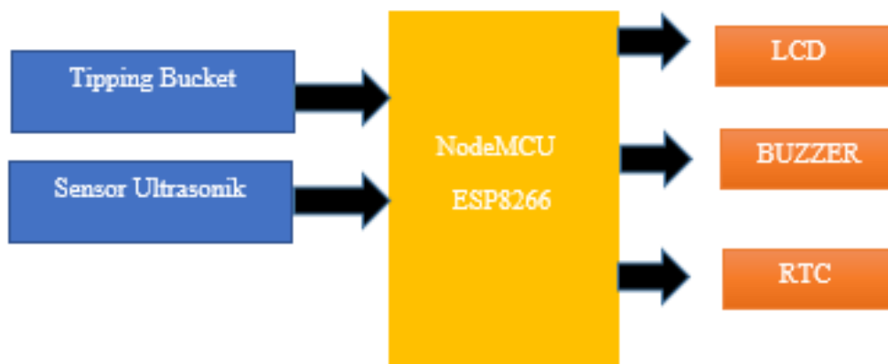
Gambar 1 Blok Diagram
