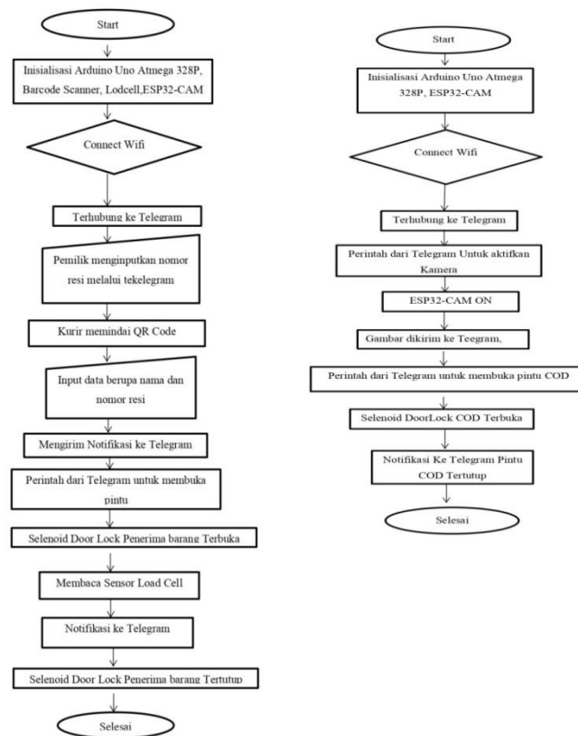
Gambar 2. Flowchart
