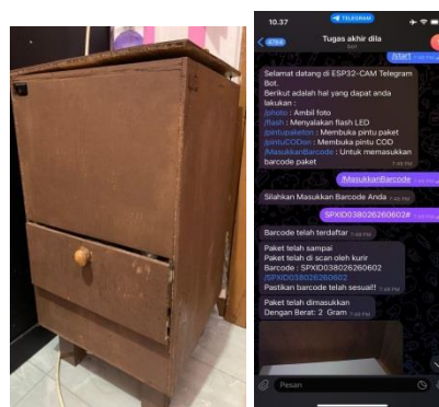
Gambar 5. Prototipe Smart Packet Box Cash on Delivery
